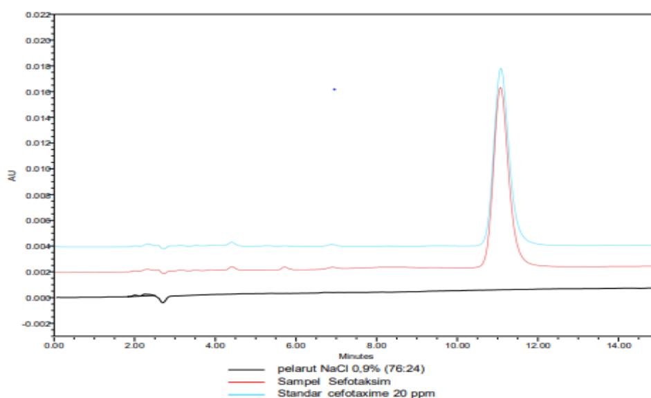
Figure 4. Specificity overlay
